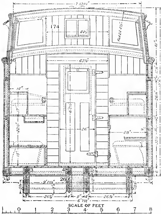
Fig. 387. Transverse Section.
